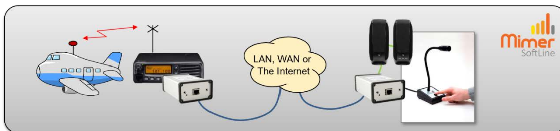
Connecting a radio at one end with a microphone and speaker at the other end, for remote control without using a PC.
