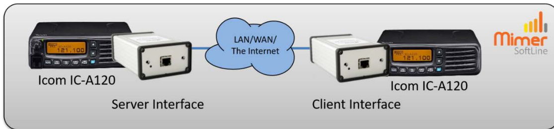
Connecting two radios of the same type back-to-back for extended coverage.
