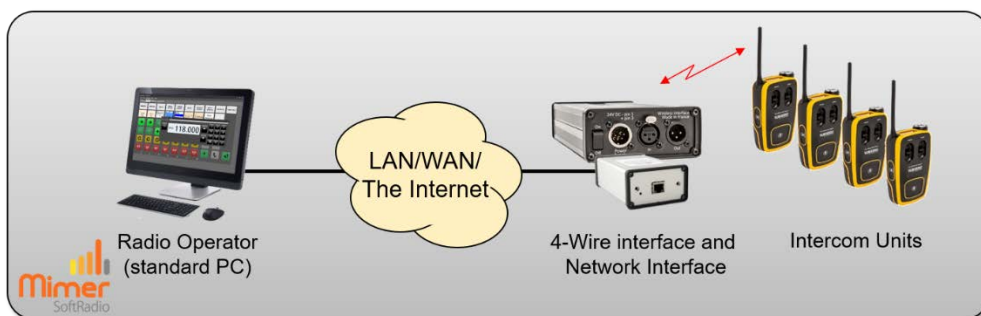
Basic setup with one operator and one Vokkero talk group
