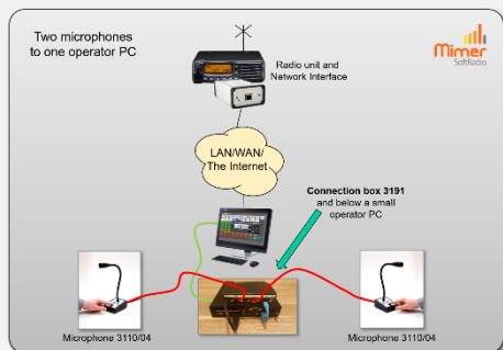
Above L.: Two microphones through a connection box to one PC.
