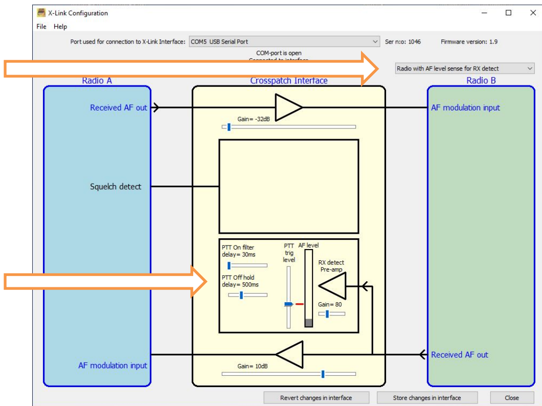
Part of the Configuration software window
